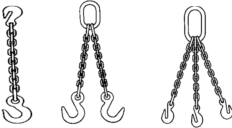
COMMON SLING HITCHES
